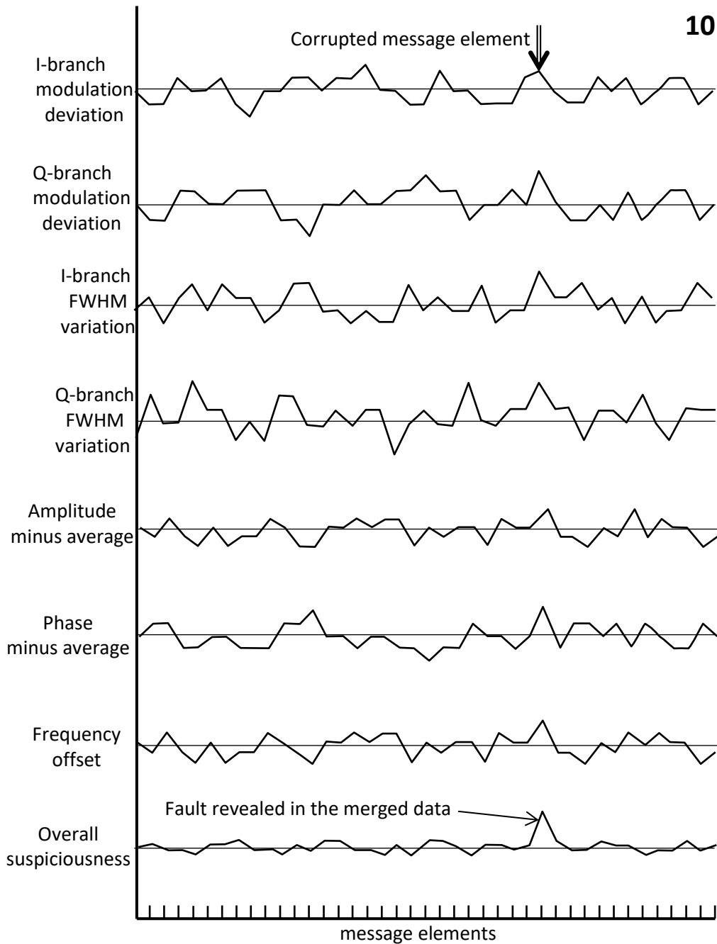
Fig. 10: Combined data reveals which message element is likely faulted. For the unfaulted message elements, measurement variations largely cancel out.
